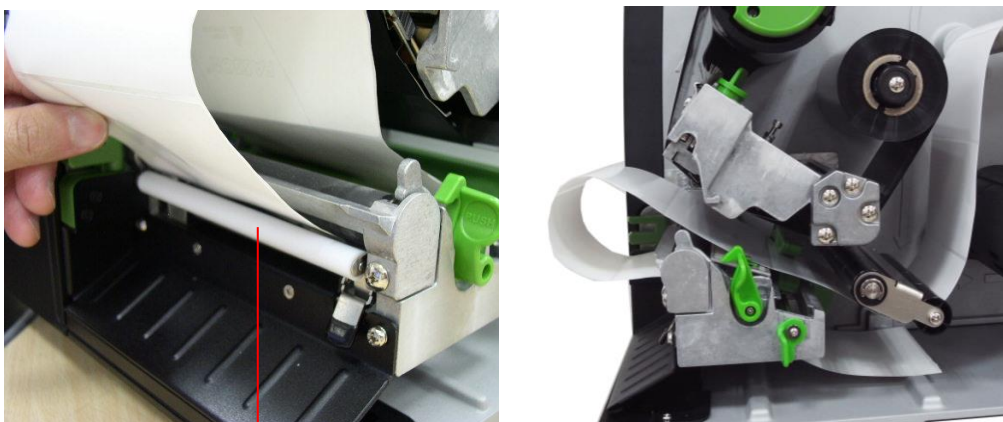
Peel-off roller
