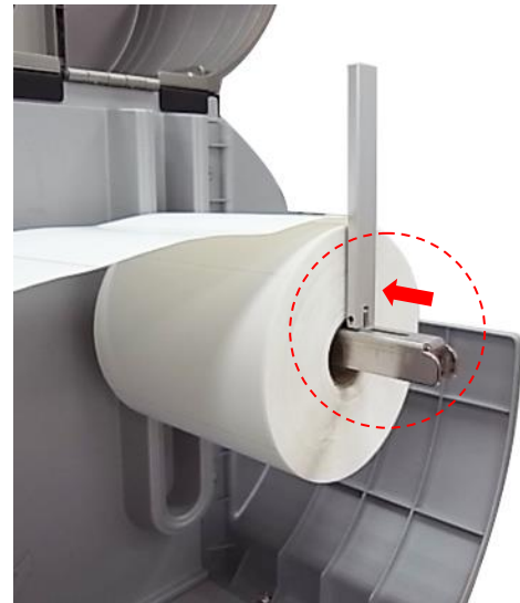
1" Label spindle
