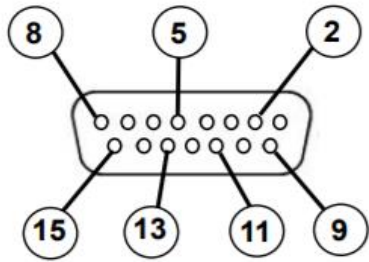
Female Connector Front View
